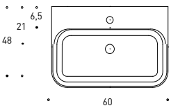
DELTA 60 ceramica / ceramic / céramique Art. A353 - P. 364
